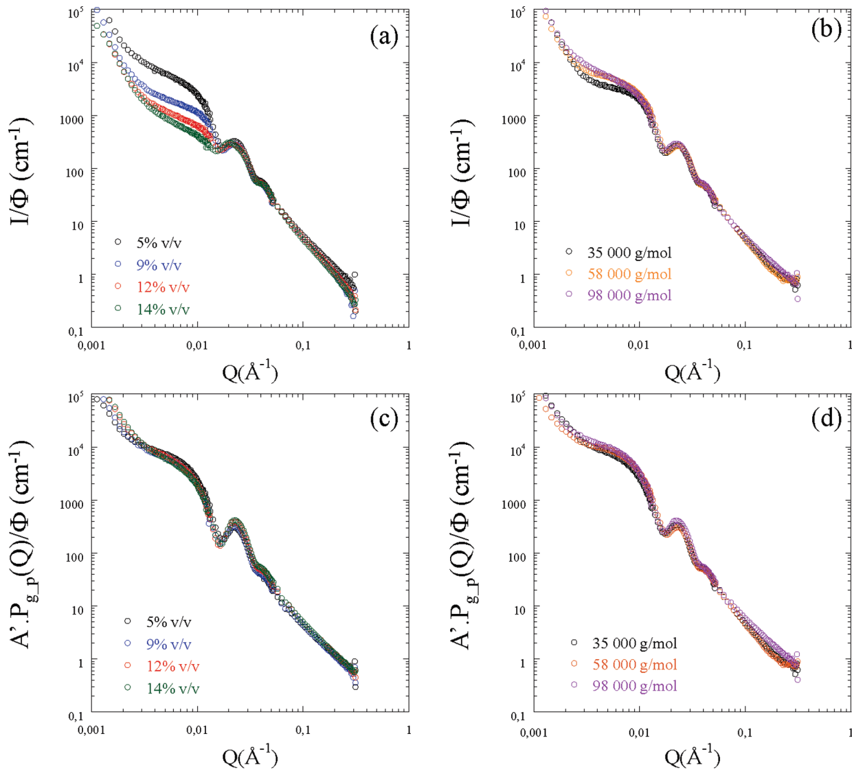
Figure 4. (a) SANS curves of the deuterated grafted corona ( M_{n,\text{grafted}} = 25\,000 g/mol) inside the silica matched matrix ( M_{n,\text{matrix}} = 98\,000 g/mol) at four particle concentrations (5, 9, 12, and 14% v/v). (b) SANS curves of the deuterated grafted corona ( M_{n,\text{grafted}} = 25\,000 g/mol) at silica volume fraction of 5% v/v inside the three silica matched matrix ( M_{n,\text{matrix}} = 35\,000 , 58 000, and 98 000 g/mol). (c) Evolution of the form factor of the grafted polymer corona in the nanocomposite P_{\text{pg}}(Q) as a function of the silica content obtained after division of the neutron scattering intensity (a) by the interparticles structure factor S_p(Q) (Figure 2c). (d) Evolution of the form factor of the grafted polymer corona in the nanocomposite P_{\text{pg}}(Q) as a function of the chain length ratio obtained after division of the neutron scattering intensity (b) by the interparticles structure factor S_p(Q) (Figure 2d).
