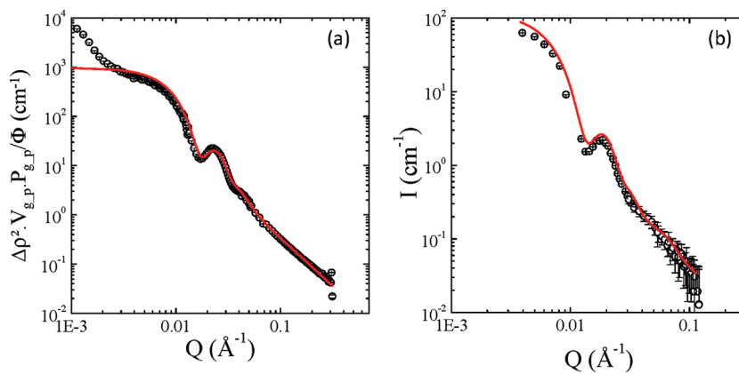
Figure 5. (a) Modelization of the form factor of the deuterated PS grafted silica nanoparticles ( M_{n,\text{grafted}} = 25\,000 g/mol) dispersed in a silica matched matrix ( M_{n,\text{matrix}} = 98\,000 g/mol) with a Gaussian chain model for comparison with the modelization of the same grafted particles dispersed in a solvent (b) and modeled with a core-shell model (from ref 11).
