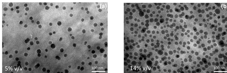
Figure 3. Transmission electronic microscopy (TEM) on the nanocomposite ( M_{n,\text{matrix}} = 98\,000 g/mol) filled with 5% v/v (a) and 14% v/v (b) of grafted silica particles ( M_{n,\text{grafted}} = 25\,000 g/mol).
